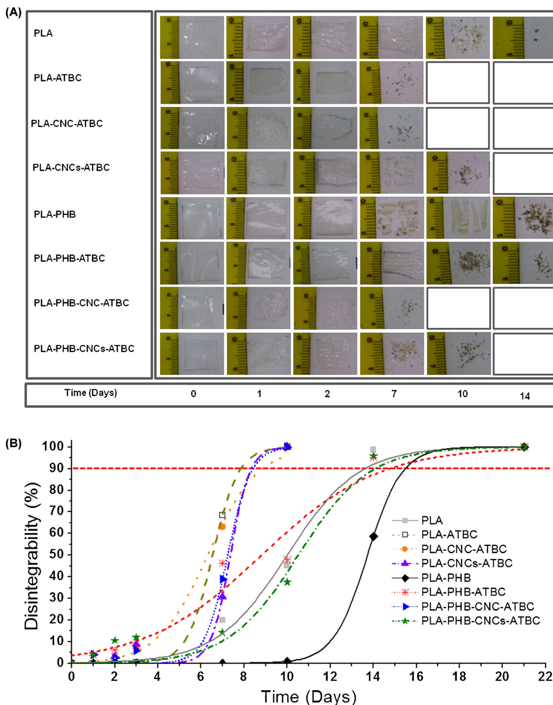
Fig. 5. (A) Visual appearance of film samples before and after different incubation days under composting conditions. (B) Film disintegration degree under composting conditions as a function of time.
