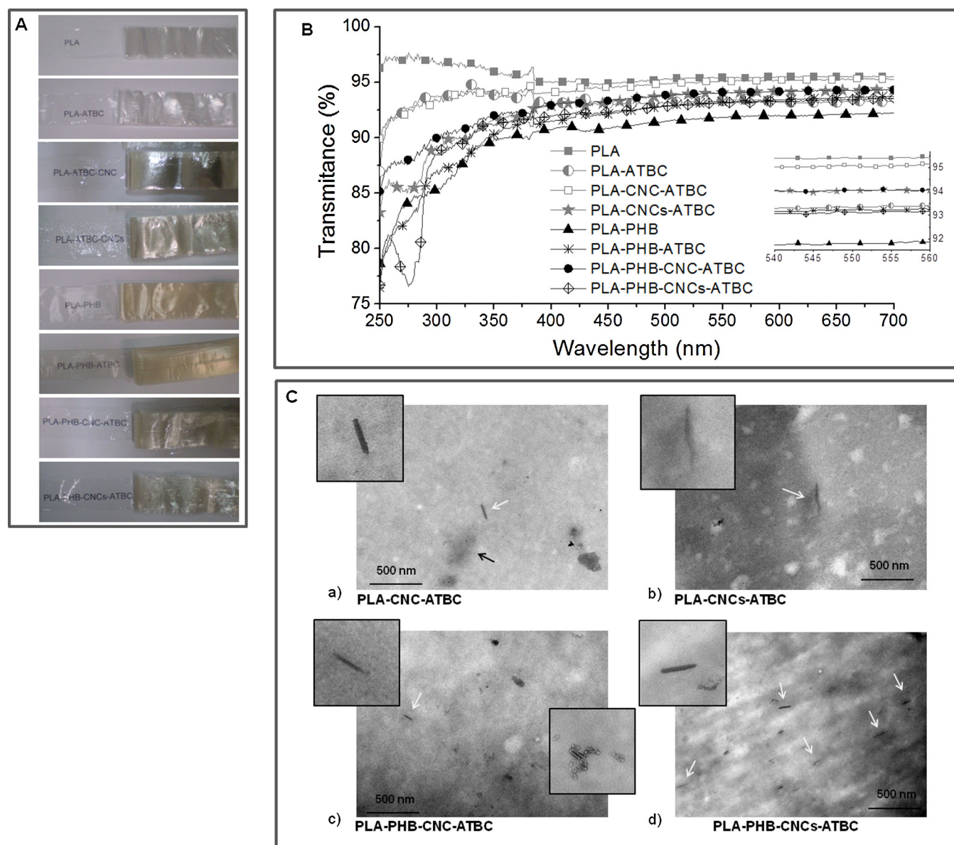
Fig. 1. Plasticized PLA, PLA-PHB and nanocomposite films: (A) visual appearance, (B) UV-vis spectra and (C) TEM analysis of nanocomposite films with cellulose nanocrystals.
