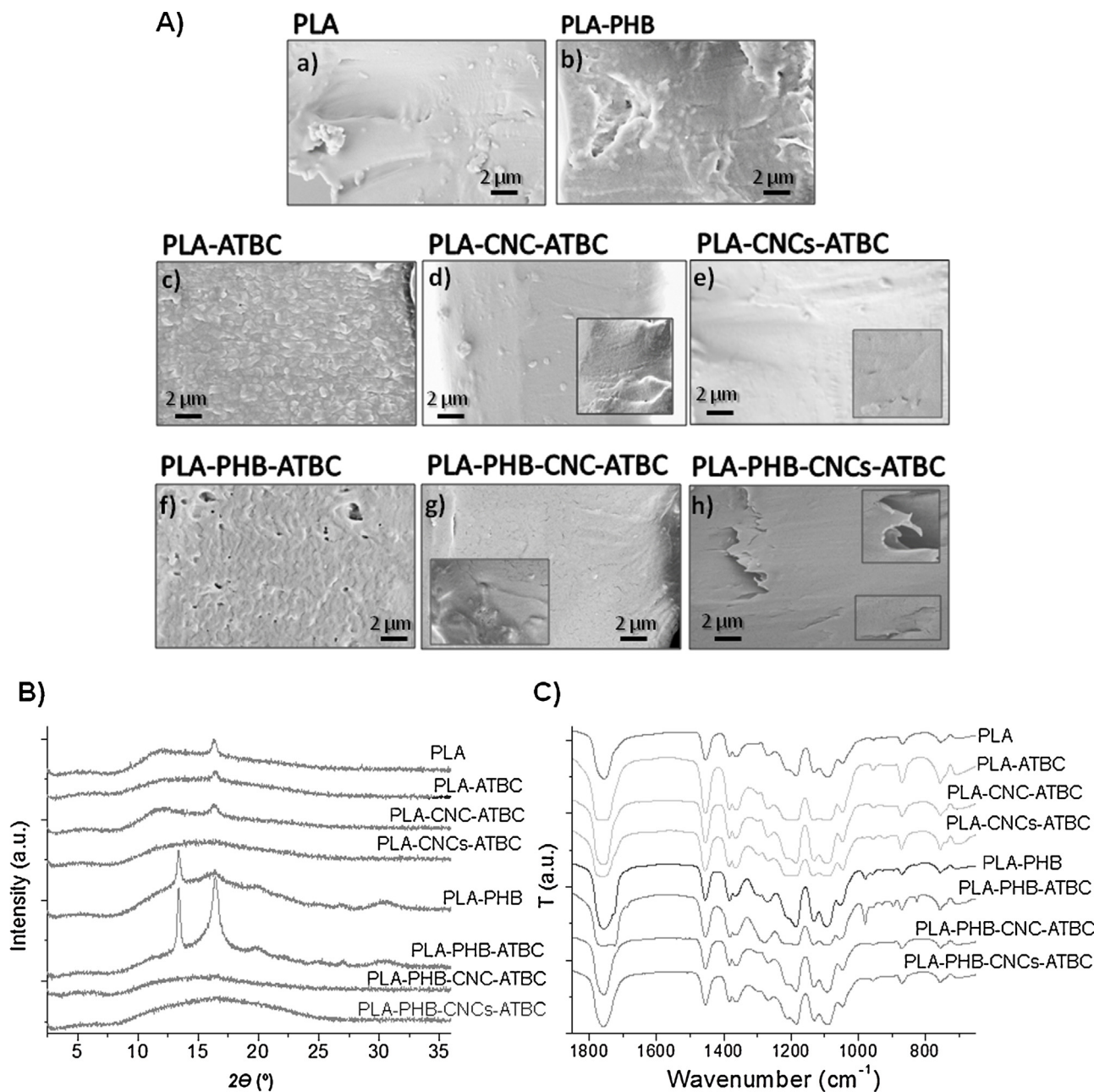
Fig. 2. Plasticized PLA, PLA-PHB and nanocomposite films: (A) microstructure of fracture surface at 20,000× magnifications and inset figure at 35,000× magnifications, (B) X-ray diffraction patterns and (C) FTIR spectra.
